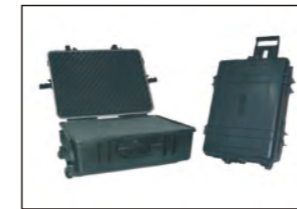
ITEM: EPC021B Material: ABS ID: L562 × W408 × H195 mm OD: L635 × W475 × H250 mm
