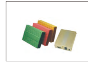
ITEM:AEH088 Material:AL SIZE:W120×H40×L100 mm
