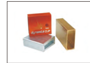
ITEM:AEH020 Material:AL SIZE:W66×H27×L100 mm
