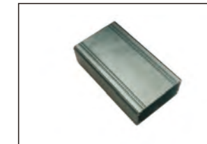
ITEM:AEH032 Material:AL SIZE:W57×H28×L100 mm
