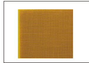
ITEM:PCB01 2.54mm pitch Hole size: 1.0mm Board thickness: 1.2mm/1.5mm
