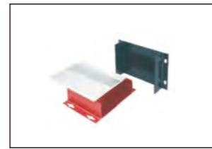
ITEM:AEH068 Material:AL SIZE:W147×H36×L100 mm
