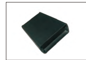
ITEM:AEH198 Material:AL SIZE:W82×H32.5×L100 mm
