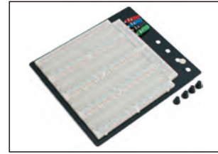
ITEM:EB03B-4S7P 3220 tie-point 7 Power lanes,700 PTS 4 Standard double-strips,2520 PTS SIZE:18.41×18.95×0.83 cm
