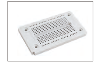
ITEM:EB08 270 tie-point 2 Power lanes,40 PTS 1 Standard double-strip,230 PTS SIZE:9.0×5.2×0.83 cm
