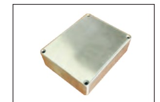
ITEM:AP004 Material:AL OD:L120×W94×H34mm WEIGHT:192g
