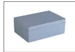
ITEM:AW058 Material:AL SIZE:L332×W232×H121.5 mm
