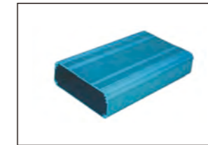
ITEM:AEH022 Material:AL SIZE:W65×H25×L100 mm
