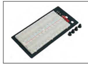
ITEM:EB03B-2S1P 1360 tie-point 1 Power lane,100 PTS 2 Standard double-strips,1260PTS SIZE:16.51×8.05×0.83 cm
