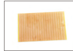
ITEM:PCB02 2.54mm pitch Hole size: 1.0mm Board thickness: 1.2mm/1.5mm
