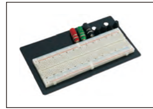
ITEM:EB03B 830 tie-point 2 Power lanes, 200 PTS 1 Standard double-strip, 630 PTS SIZE:16.51×5.45×0.83 cm
