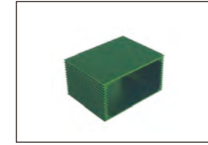
ITEM:AEH087 Material:AL SIZE:W111.5×H58×L100 mm
