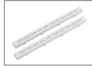
ITEM:EB04-2P 200 tie-point 2 Power lane,200 PTS SIZE:17.12×1.25×0.83 cm
