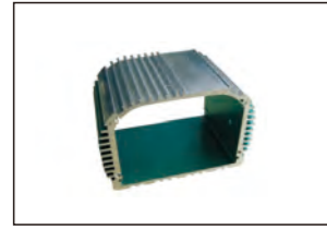
ITEM:AEH047 Material:AL SIZE:W108×H71×L100 mm
