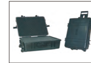
ITEM: EPC020 Material: ABS ID: L590 × W420 × H190 mm OD: L670 × W500 × H240 mm
