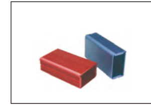
ITEM:AEH081 Material:AL SIZE:W80×H45×L100 mm
